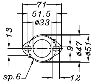
Flange "138A"
